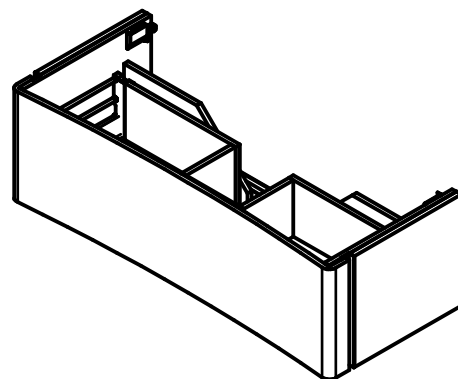
5303-WAL 1194x360x494
